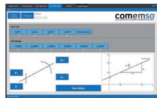
GUI recalibration
