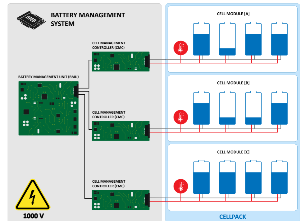
Fig. 2 Battery management
